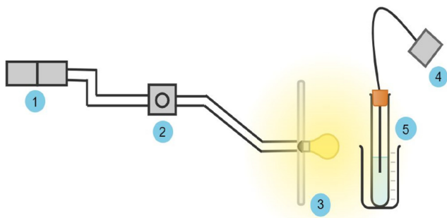
Fig. A2 The solar radiation test rig.
