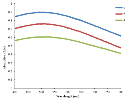
Fig. A6 UV-vis absorption of trihybrid nanofluids of t1 , t2 and t3 .
