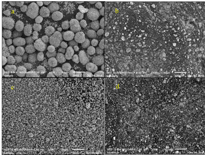
Fig. A5 Surface morphology of (a) CuO, (b) SiO 2 , (c) TiO 2 and (d) trihybrid (CuO/SiO 2 /TiO 2 ) at 300× magnification (50 μm).
