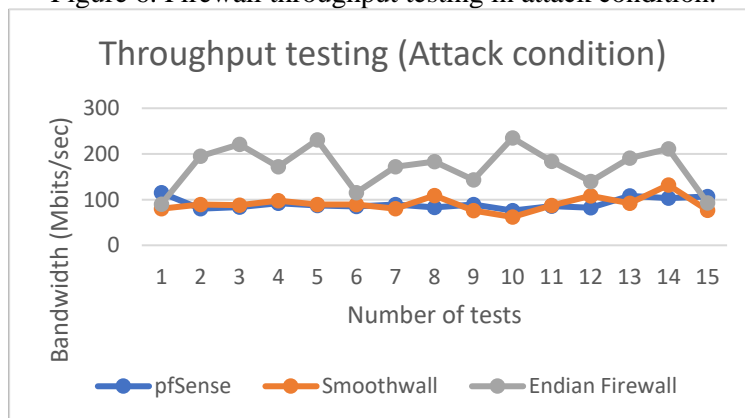
Figure 6. Firewall throughput testing in attack condition.
