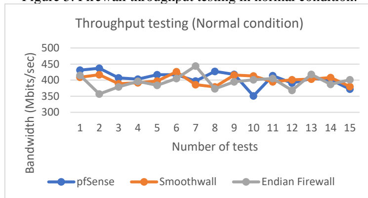
Figure 5. Firewall throughput testing in normal condition.
